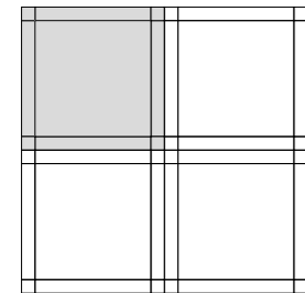
Modulo A _Module A_Modul A_Module A 4 PEZZI 7x60 (30,68%) 4 PEZZI 7x7 (3,58%) 1 PEZZO 60x60 (80,20%)
